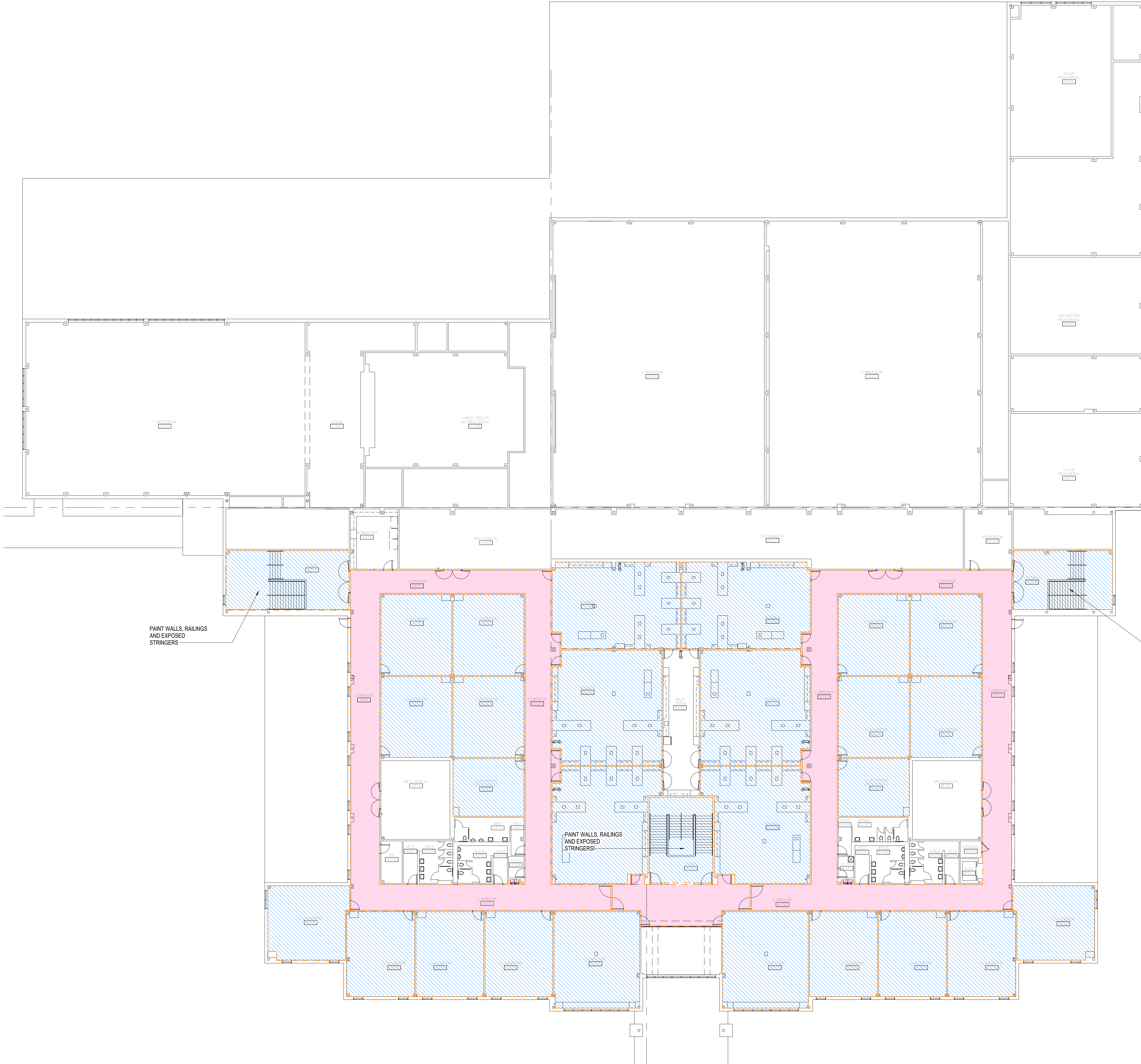
1 SOUTHMORE INTERMEDIATE SCHOOL - LEVEL 2 FLOOR PLAN 1/16" = 1'-0"
